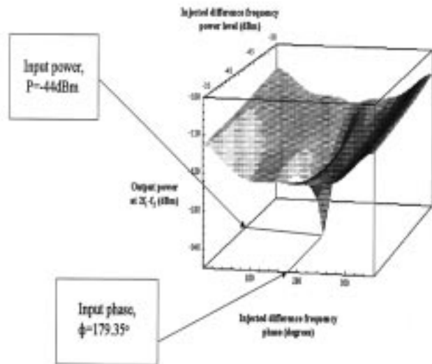
Fig. 9. IM3 ( 2f_1 - f_2 ) output power level as function of difference-frequency signal phase and amplitude.
